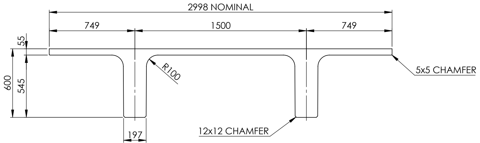
600mm DOUBLE TEE SECTION
