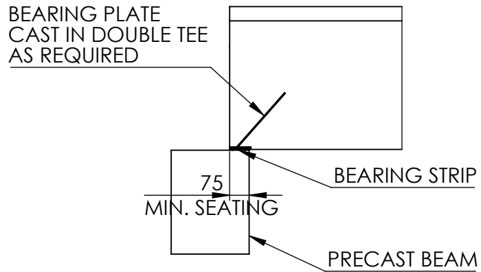
LEG SUPPORT
