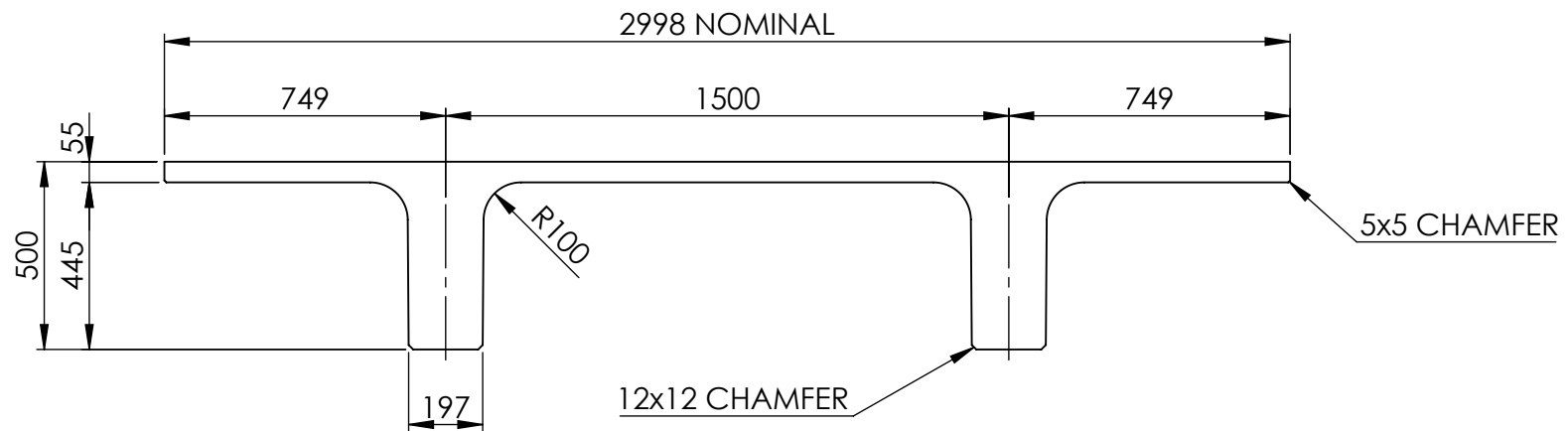
500mm DOUBLE TEE SECTION
