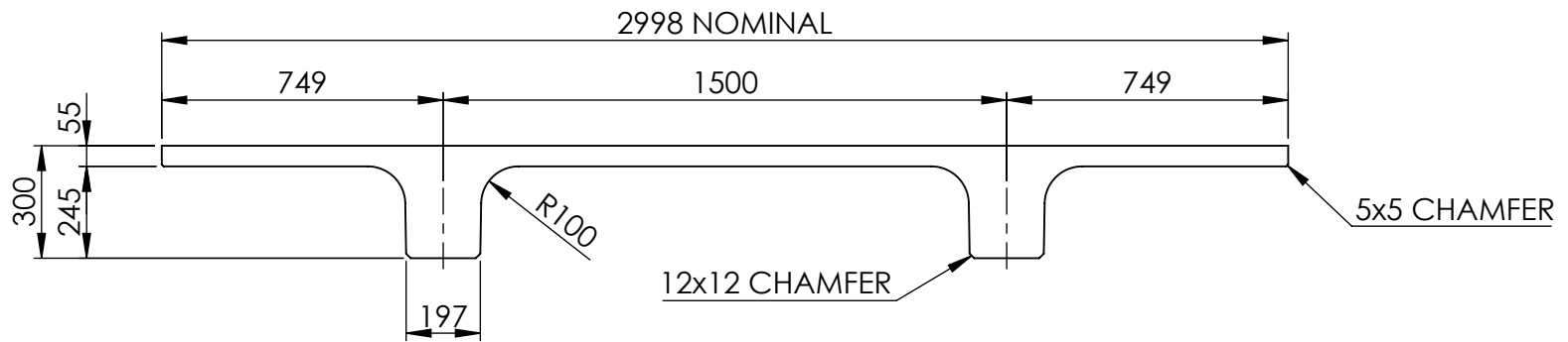
300mm DOUBLE TEE SECTION
