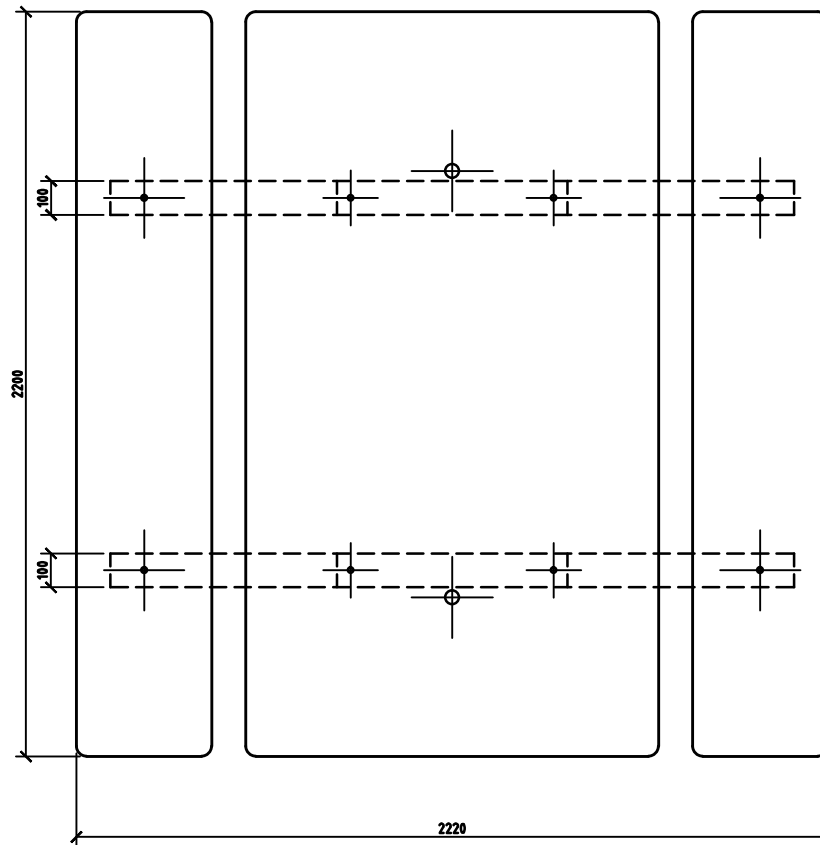
PLAN SCALE 1:5
