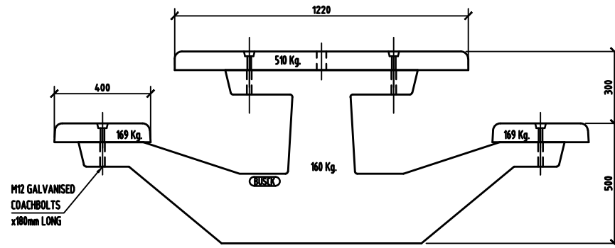
ELEVATION SCALE 1:5
